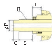
PU203~PU205 (Drawbar connection)
