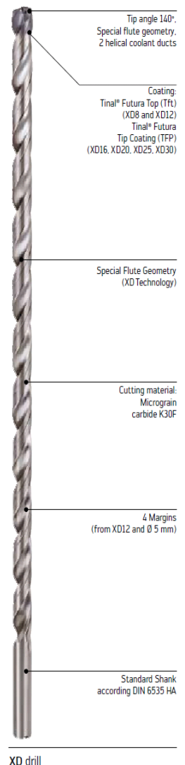
XD drill
